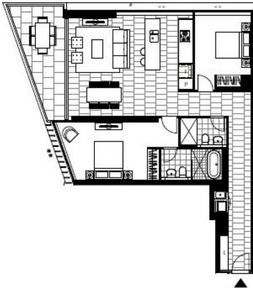
LEVEL 3, 4
